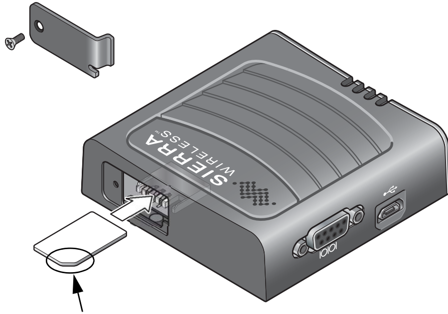
Figure 2-5: SIM Card Installation
